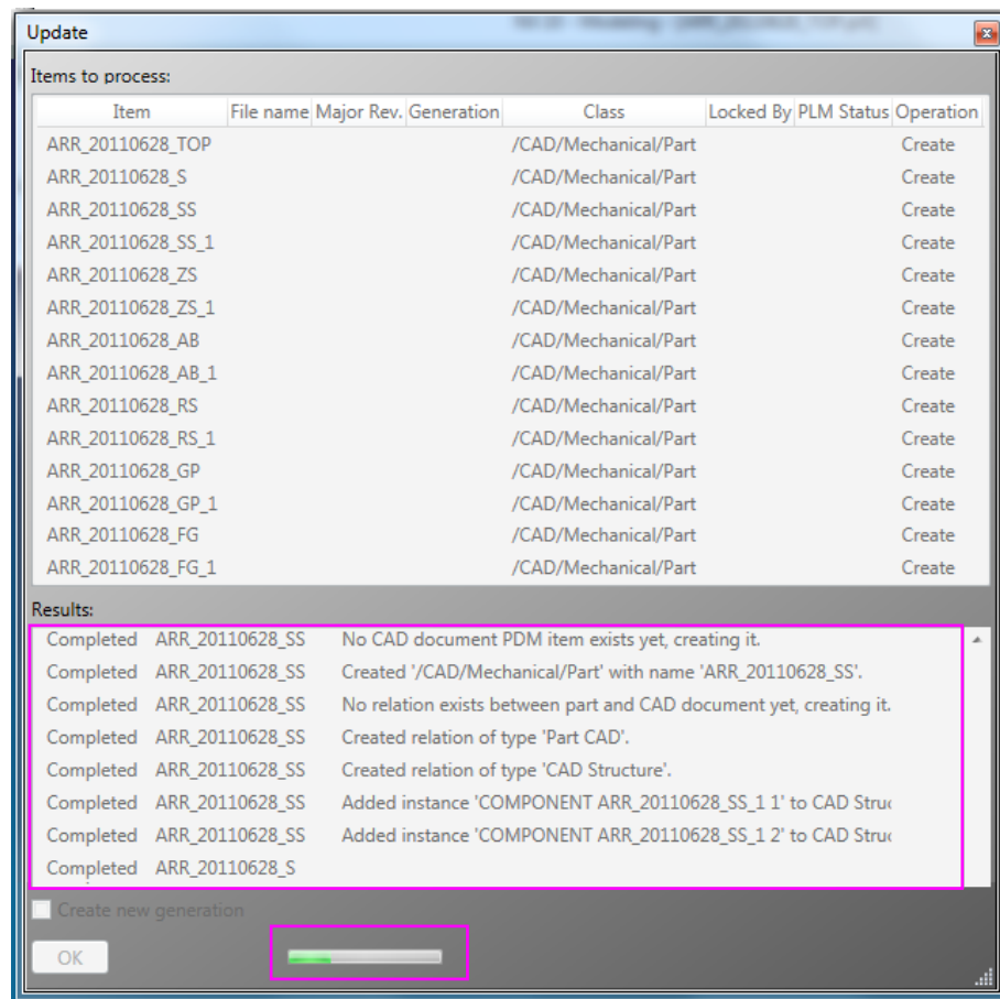
Picture 35: "Update" dialog – result and progress
