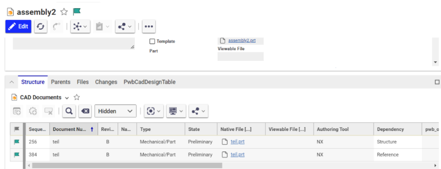
Picture 54: CAD Document item with CAD Structure / Reference relation
