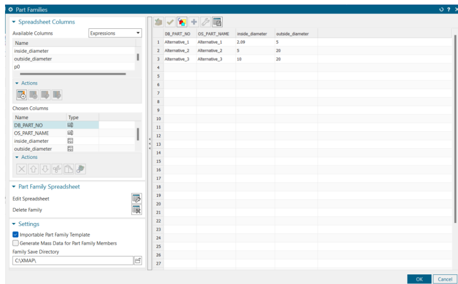
Picture 48: “Part Families” definition dialog
