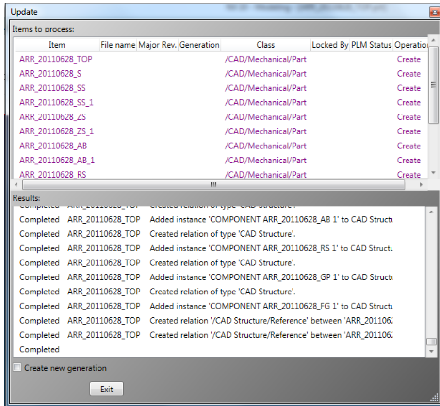
Picture 36: "Update" dialog – finished
