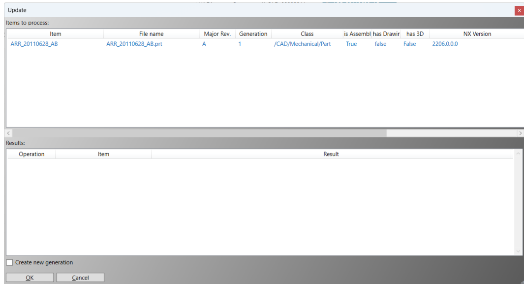
Picture 31: "Update" dialog – update and skip operations
