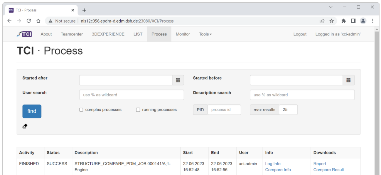
Figure 47: TCI Web – Process – Structure Compare Process Status
