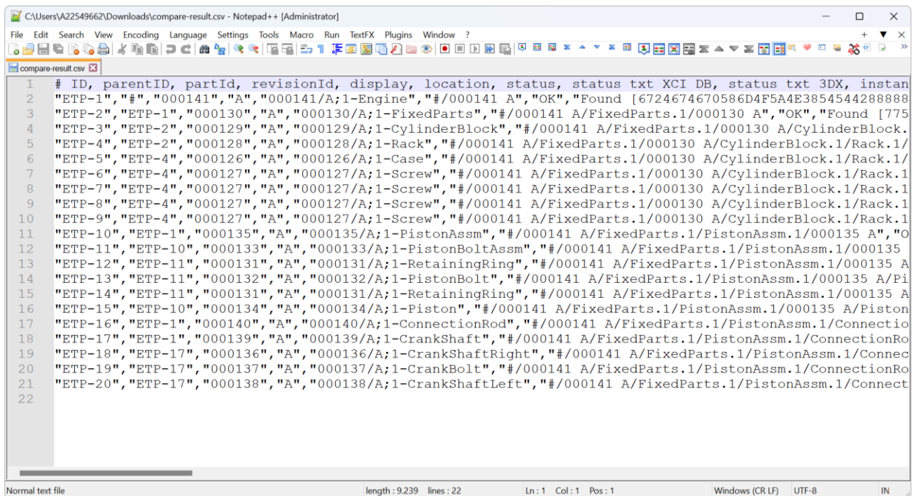
Figure 49: TCI Web – Structure Compare .csv result
