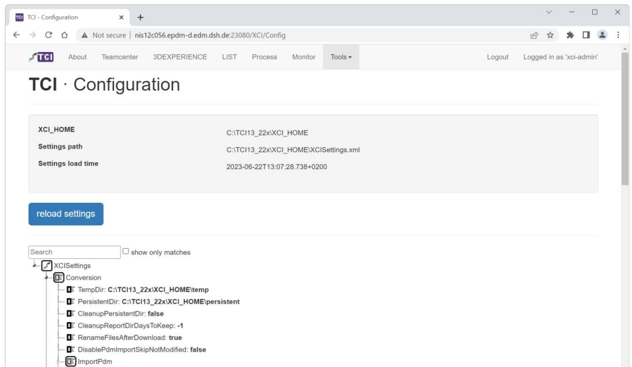
Figure 80: TCI Web – Tools – Configuration
